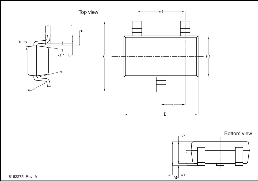
Figure 23. SOT23-3L drawing
