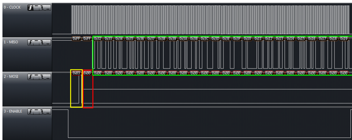
Figure 4-6. Waveform Graph 2
