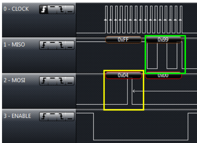
Figure 4-7. Waveform Graph 3
