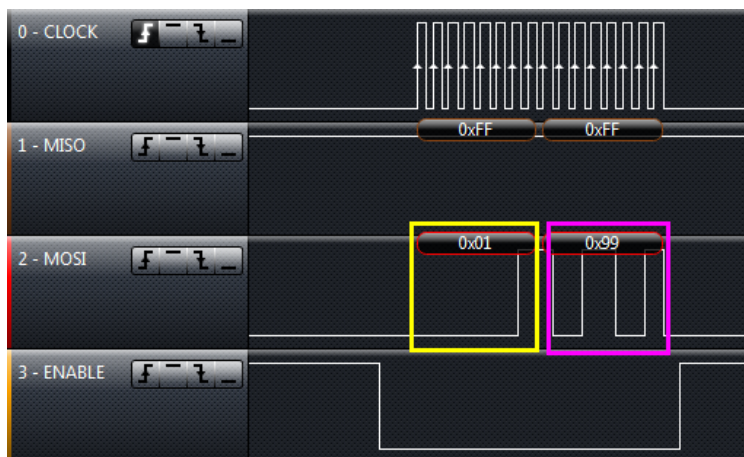
Figure 4-8. Waveform Graph 4
